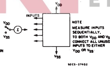
Fig. 11 - Input current.
